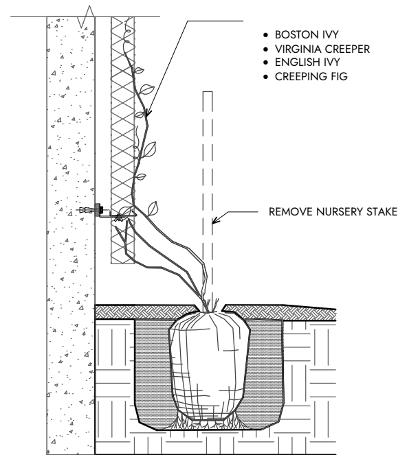
SECTION
