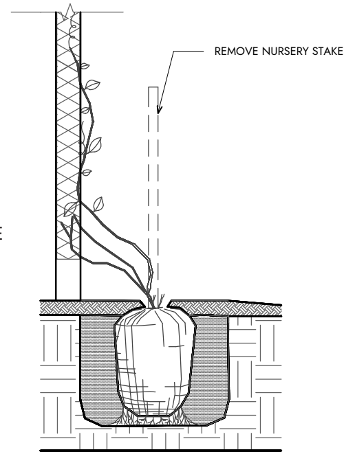
SECTION
